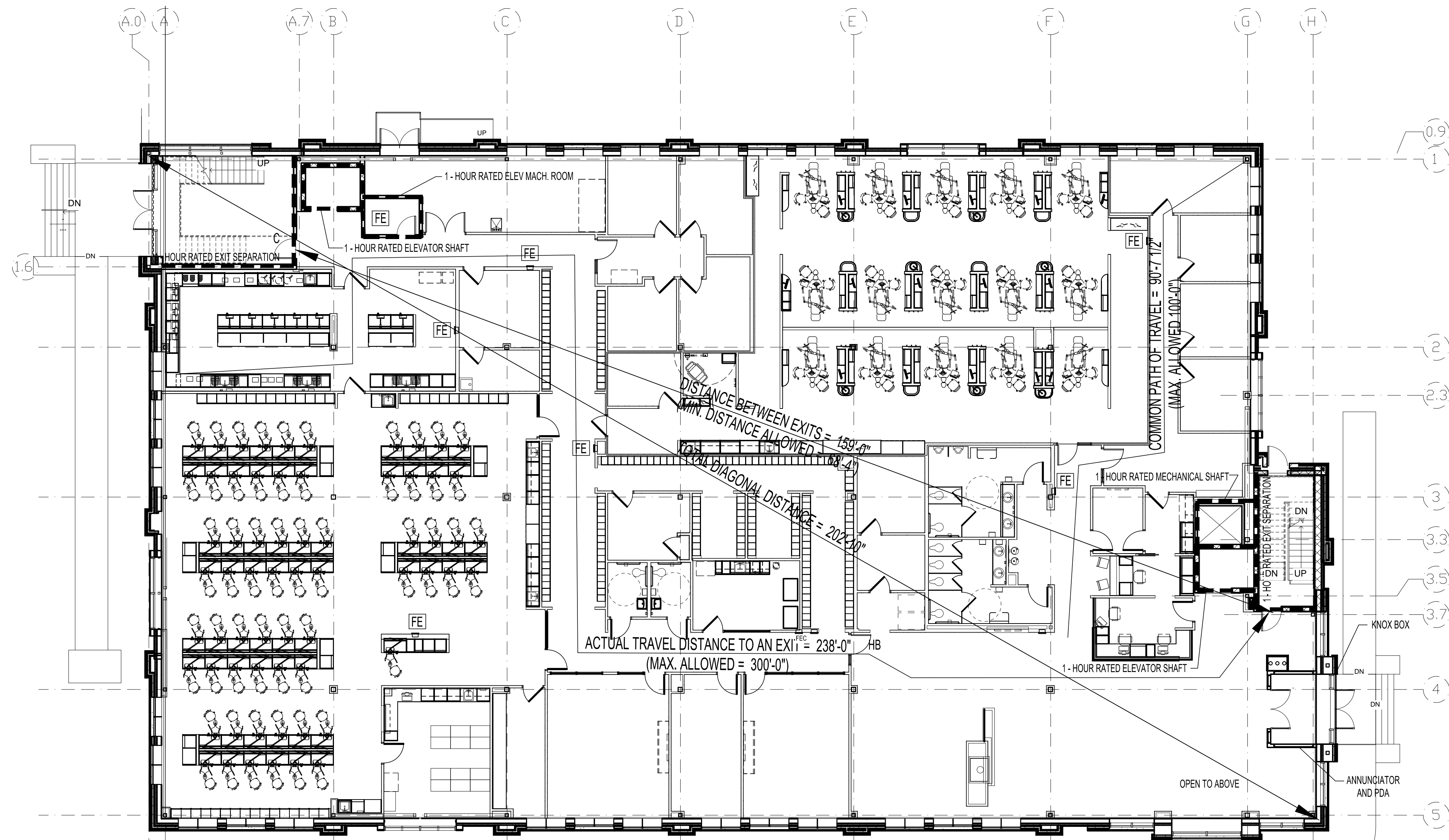
1 FIRST LEVEL EGRESS PLAN SCALE: 3/32" = 1'-0"
